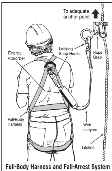
Full-Body Harness and Fall-Arrest System
